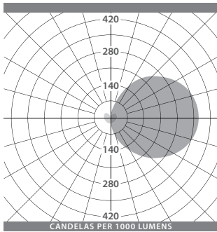
15/23W LED - PLAIN VERSION
