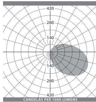
18W LED - HOOD VERSION
